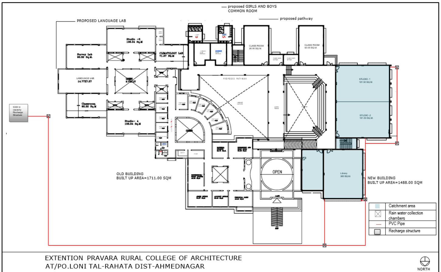
Rain water harvesting Plan
