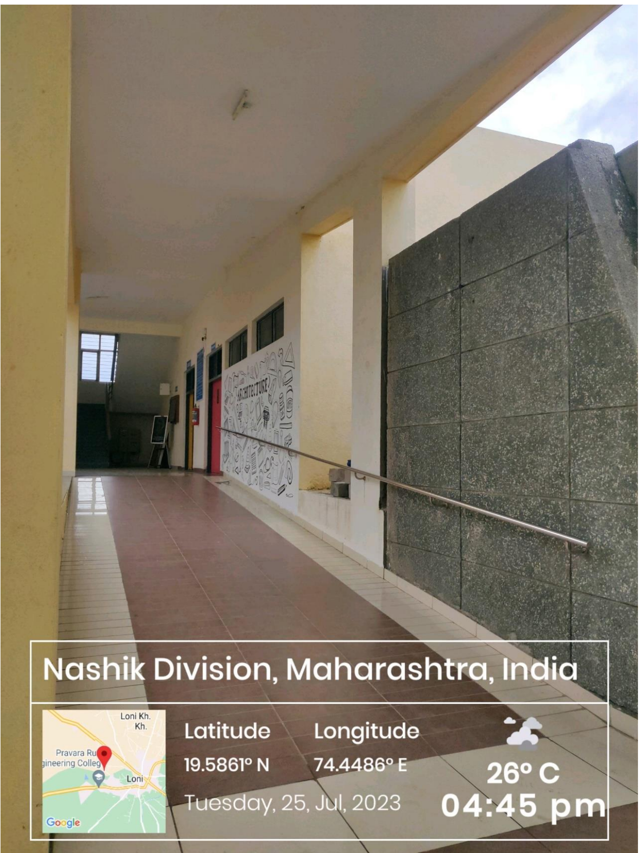
Ramp provided at new building which connects Entrance lobby to Library and classroom
